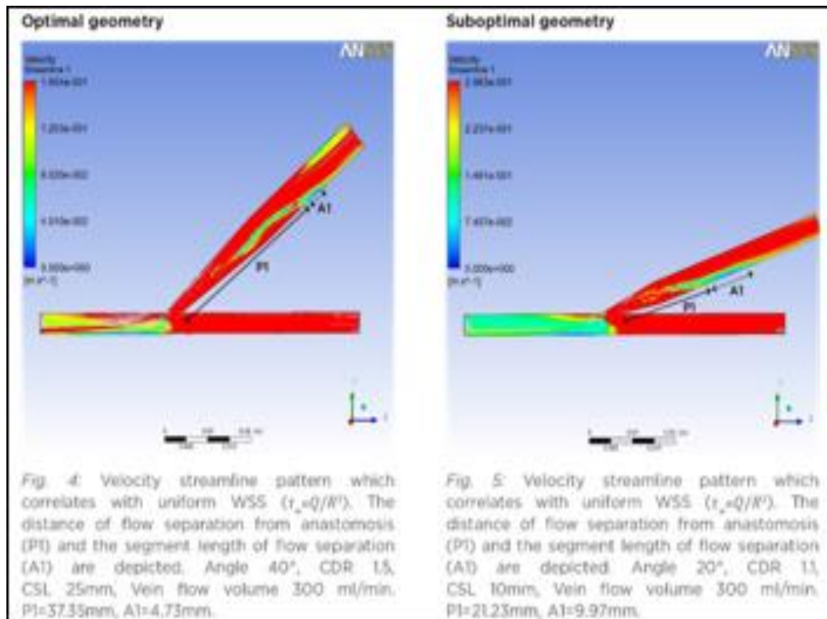
Velocity streamline patterns optimal vs suboptimal anastomotic geometry
