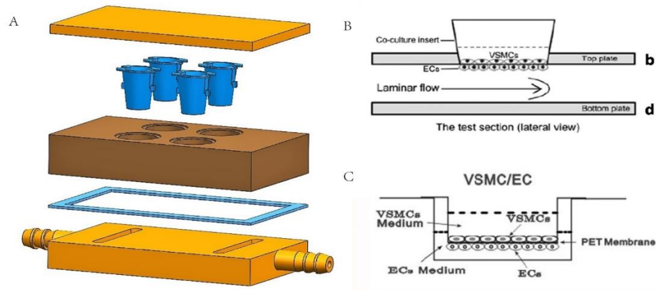
EC/VSMC cocultured parallel-plate flow chamber system.
