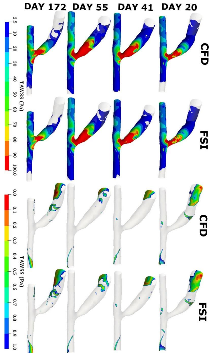
Contour plots of high and low TAWSS distributions, calculated by CFD and FSI, display similar distribution patterns.
