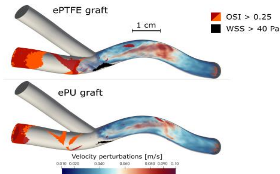
Figure 1: Overview of the magnitude of venous turbulent velocity perturbations and the venous areas exposed to high OSI ( >0.25 ) or very high ( >40 Pa) WSS for the ePTFE (top) and ePU (bottom) graft. Note that the red regions denote high OSI on the front of the geometry, whereas the orange regions denote high OSI on the back of the geometry.
