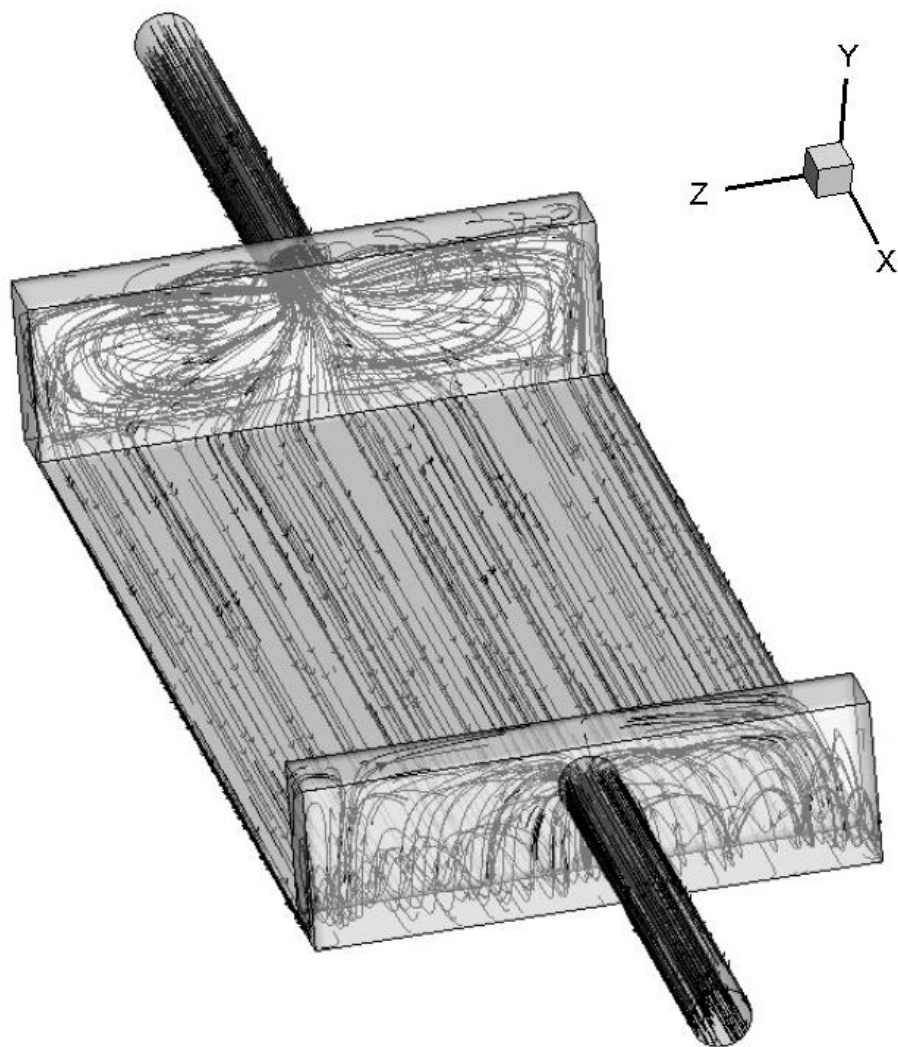
Distribution of the flow in parallel-plate flow chamber
