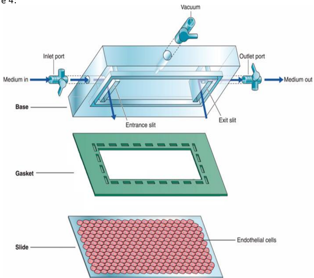
Diagram showing the parallel-plate flow chamber (From Chiu JJ, et al)
